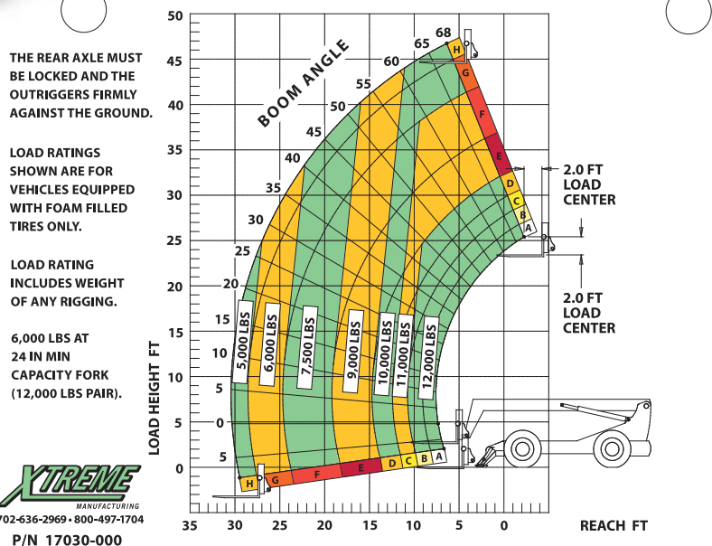
XR1245 LOAD CHART OUTRIGGERS DOWN- STANDARD CARRIAGE
